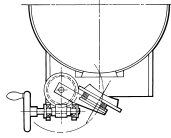
Flush Plug Valve - equipped for manual or pneumatic operation, this valve eliminates dead spots in the blender trough
